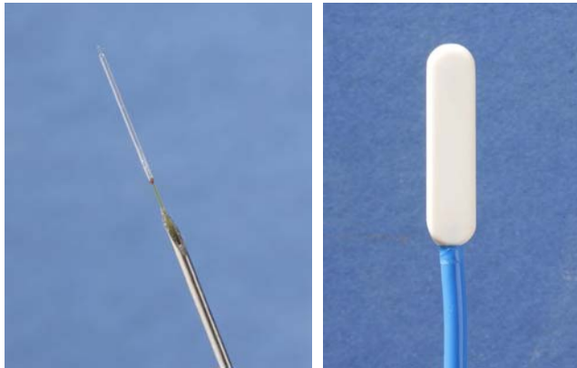
Fig. 2. Bare (left: in a gage 24 hypodermic needle) and packaged (right) FOT-L temperature sensor is suitable for skin temperature monitoring of patients that are under extreme magnetic field during MRI procedures.
