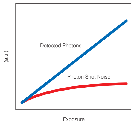
Figure 2: Detected photons and photon shot noise: sub-linear relationship.
